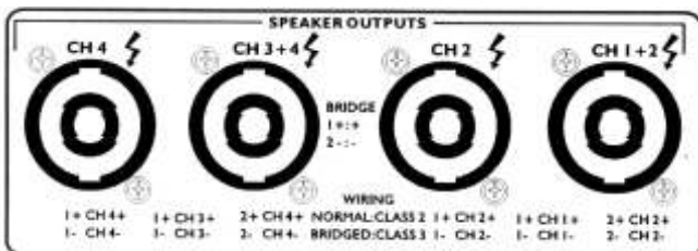
Speakon outputs-4-channel models
