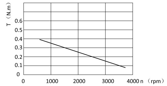
Torque--speed characteristic
