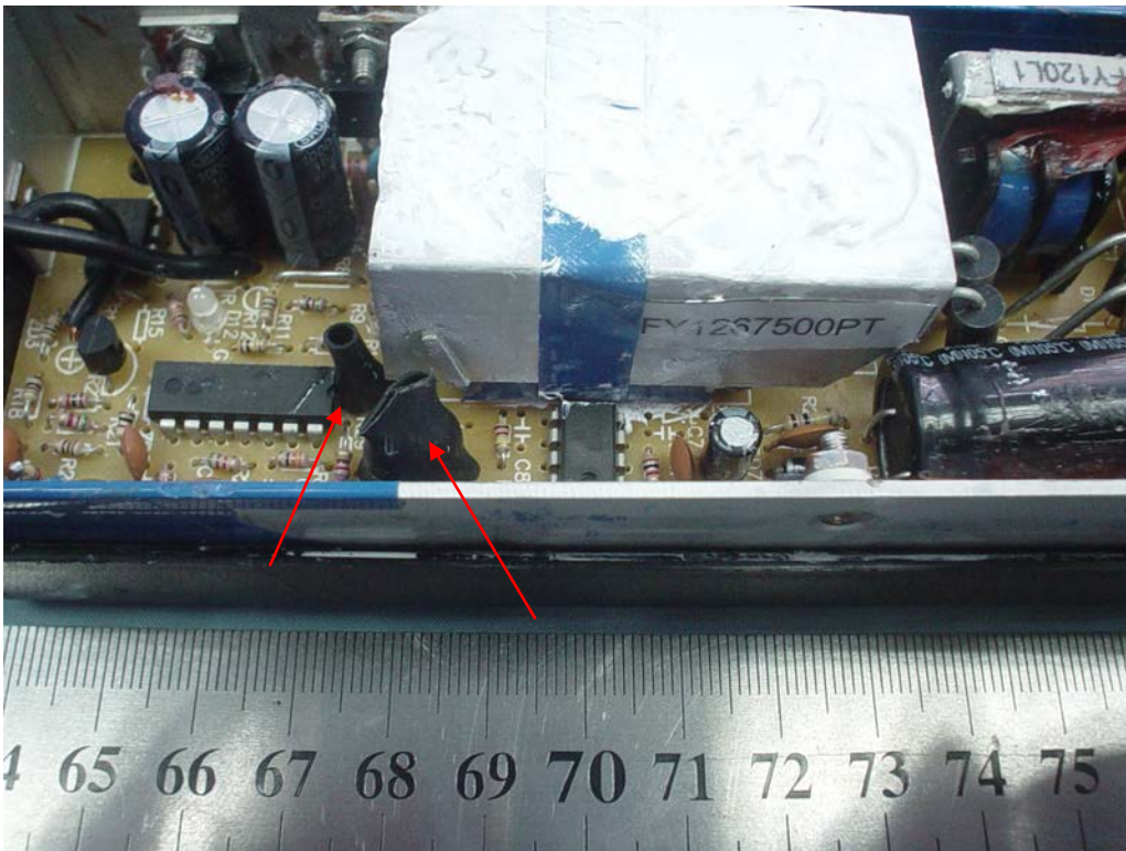
Figure 12. heat shrinkable tube on C9 and C11
