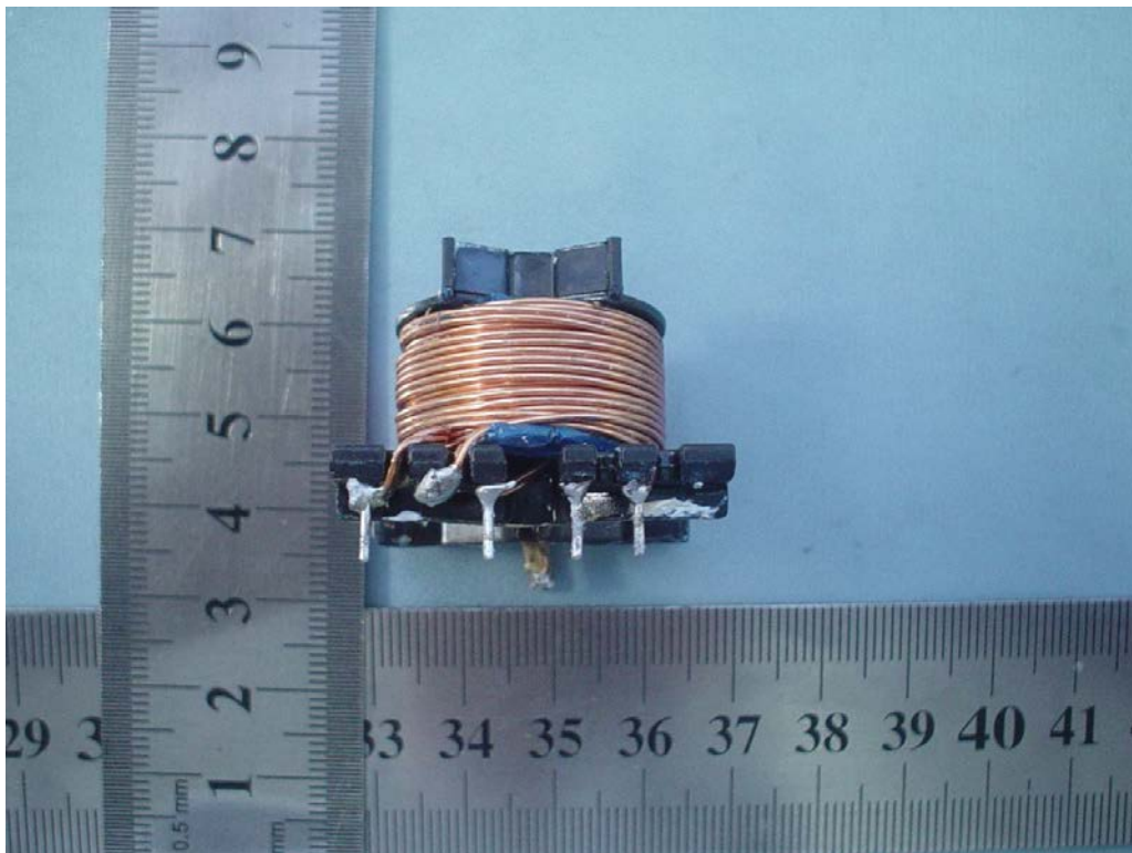
Figure 10. primary winding
