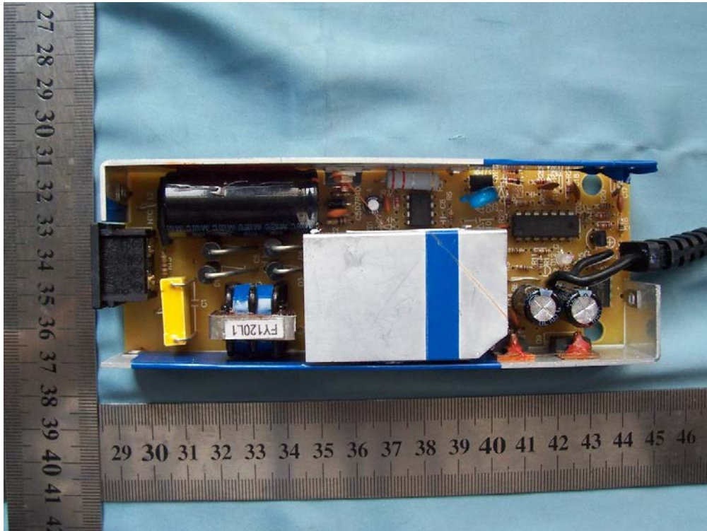
Figure 5. front view of PCB
