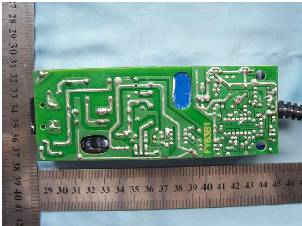
Figure 6. back view of PCB
