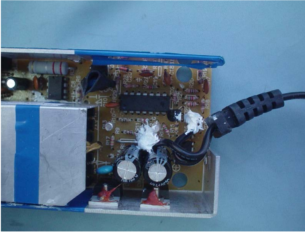
Figure 13. glue for fixing output wire
