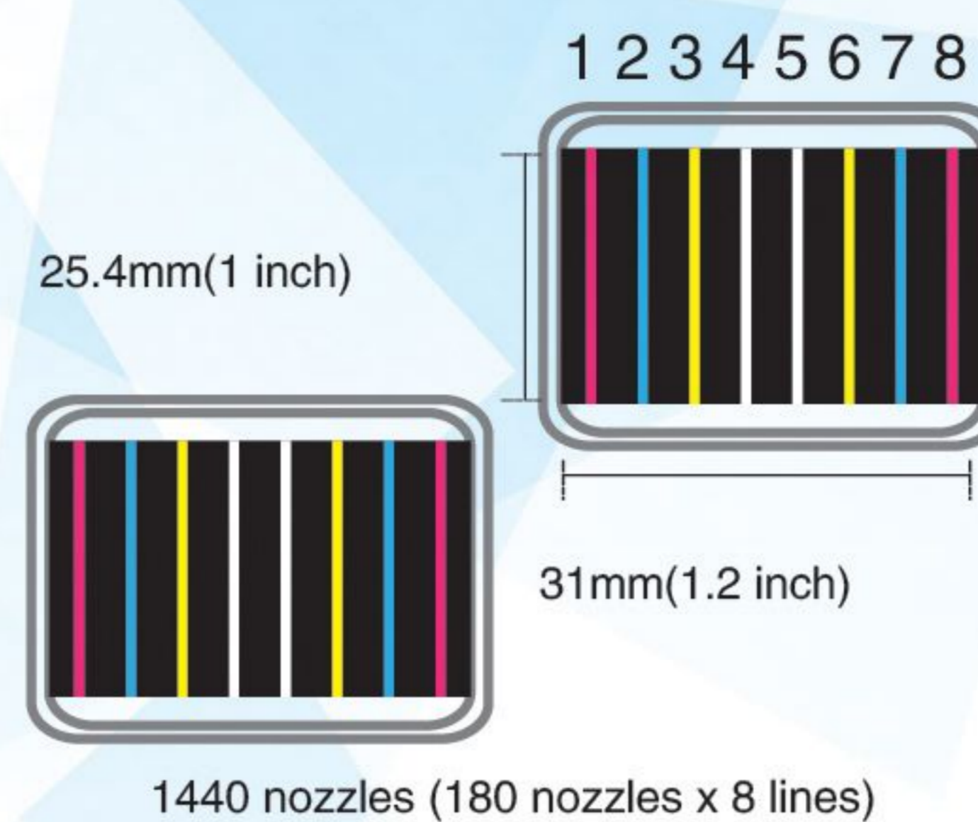
Piezoelectric Print Head Variable Ink Droplet
